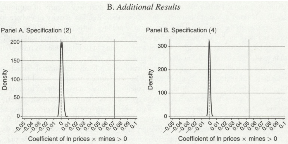
FIGURE 4. MONTE CARLO SAMPLING DISTRIBUTION OF (\ln \text{ price} \times \text{mines} > 0)
