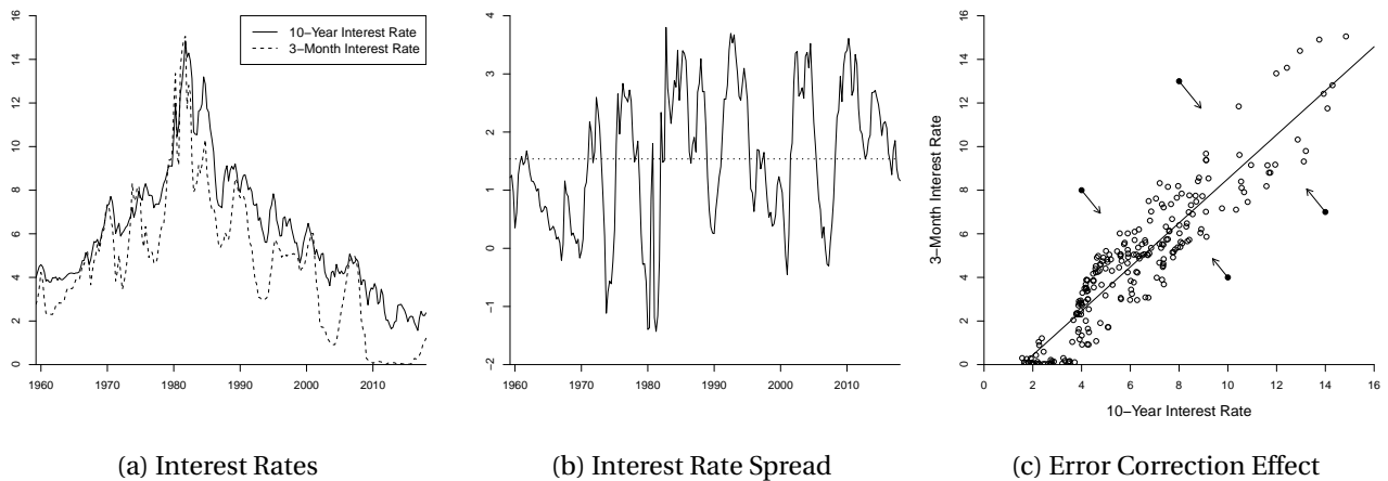
Figure 16.6: Cointegration
