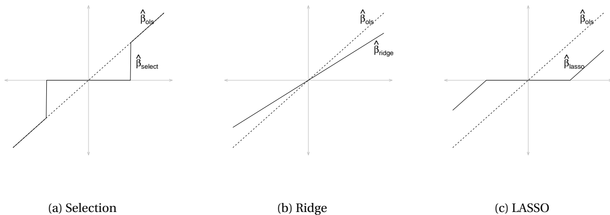
Figure 29.4: Transformations of least squares coefficients by Selection, Ridge, and LASSO estimators
