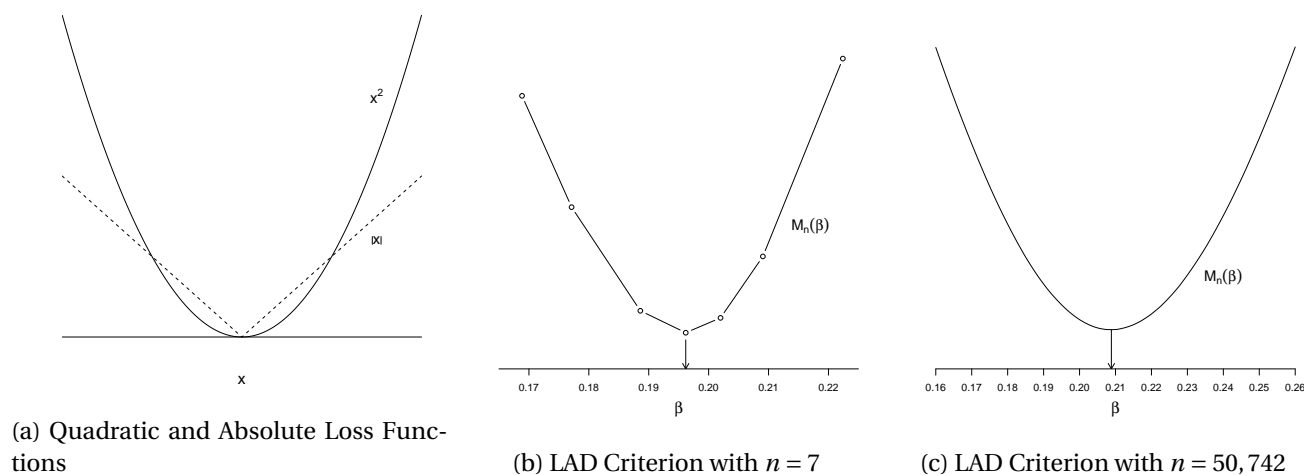
Figure 24.1: LAD Criterion
