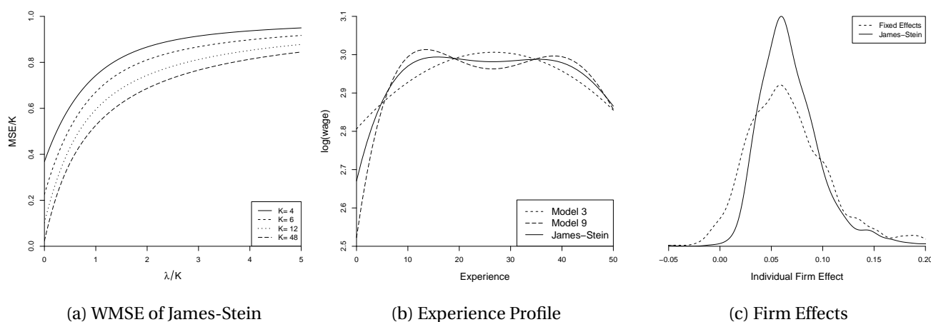
Figure 28.3: James-Stein Estimator
