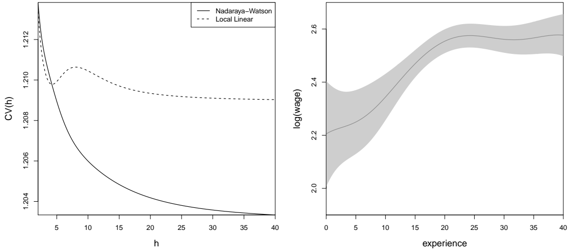
(a) Cross-Validation for Conditional Variance
