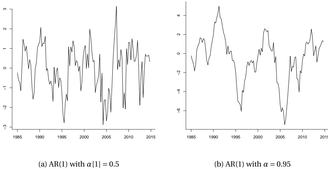
Figure 14.6: AR(1) Processes
